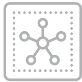
Vehicle Sharing
